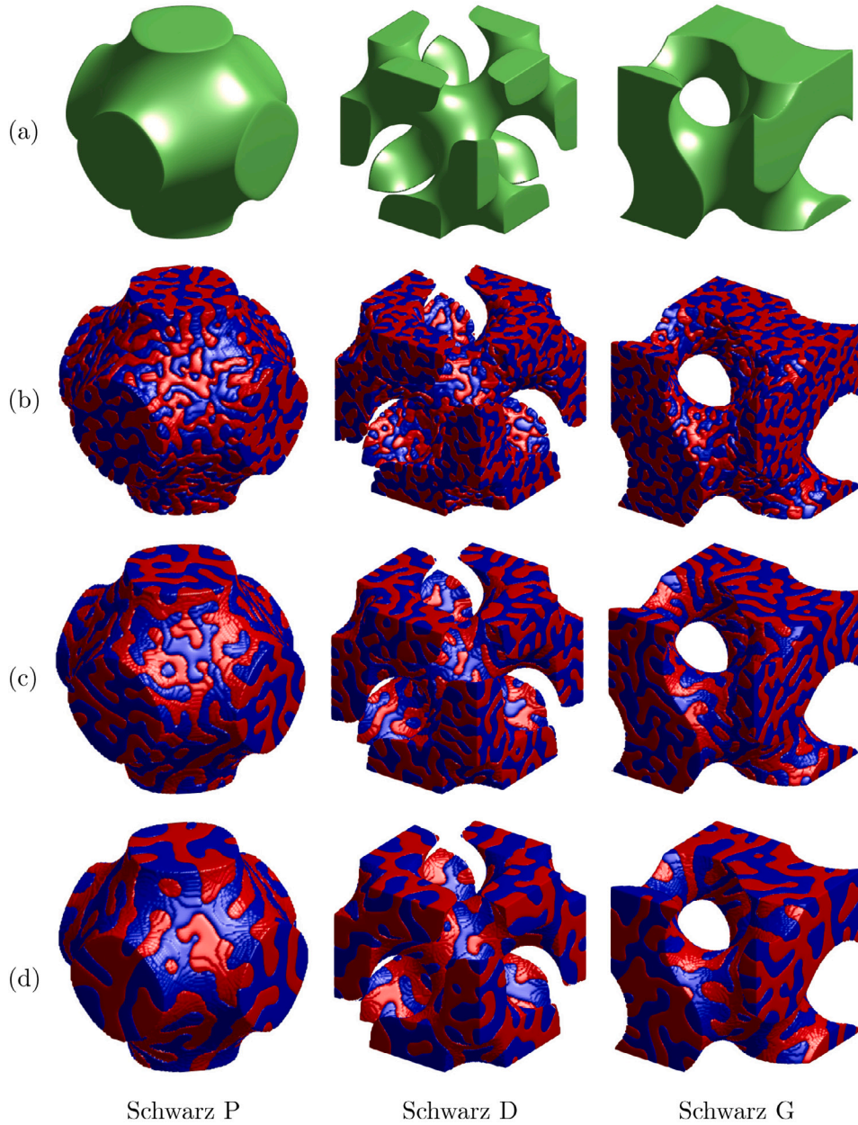
Fig. 19. 3D phase separation in complex domains. Here, the Schwarz P, Schwarz D, and Schwarz G domains are shown in the left, middle, and right columns of (a). From (b)–(d), the snapshots are at t = 0.0059, 0.0352 , and 0.1113 . The red and blue regions are occupied by two different components. With time evolution, the co-continuous patterns can be observed. (For interpretation of the references to color in this figure legend, the reader is referred to the web version of this article.)
