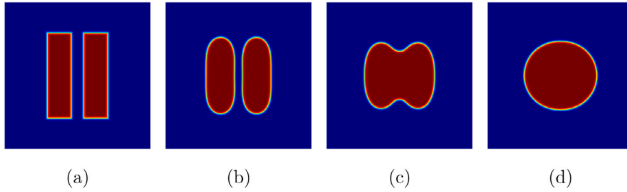
Fig. 3. Evolution of initially separated components with sharp shapes. From (a)–(d), the snapshots are at t = 0, 1.56, 3.13, \text{ and } 11.72 . Because the CH model dissipates the free energy by minimizing the interfacial length, the sharp corners become smooth and finally merge with each other to form the circular shape.
