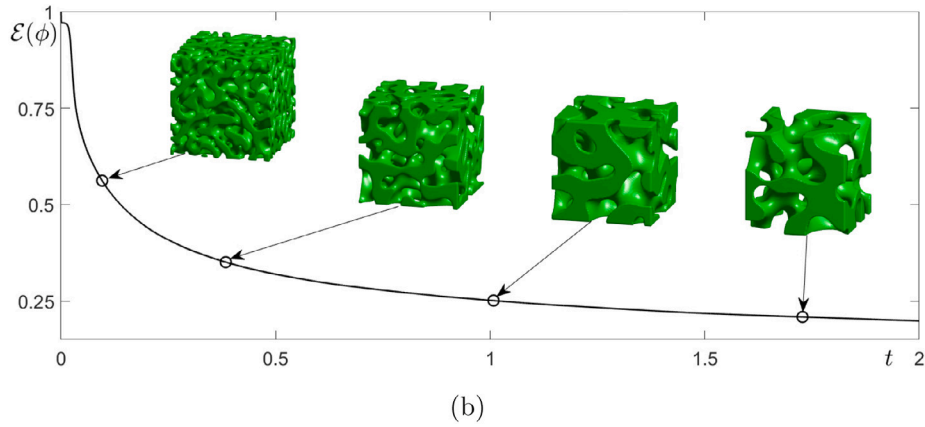
Fig. 15. Evolutions of discrete energy functional with respect to different average concentrations: (a) \bar{\phi} = -0.4 and (b) \bar{\phi} = 0 . Here, the solid lines represent the energy curves, the open circle markers represent the specific moments. The insets show the snapshots of zero level set of \phi at t = 0.096, 0.384, 1.008 , and 1.728 (from the left to right). The energies are decreasing with the evolutions of phase coarsening.
