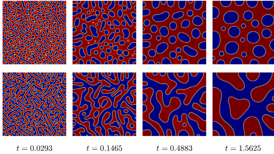
Fig. 10. Snapshots with respect to \bar{\phi} = 0.2 (the top row) and \bar{\phi} = 0 (the bottom row). The computational moments are illustrated under each figure. With even concentration (i.e., \bar{\phi} = 0 ), the co-continuous pattern evolves. On the contrary, the droplet patterns can be observed when one component is dominant. These coarsening processes occur due to the minimization of free energy of the system.
